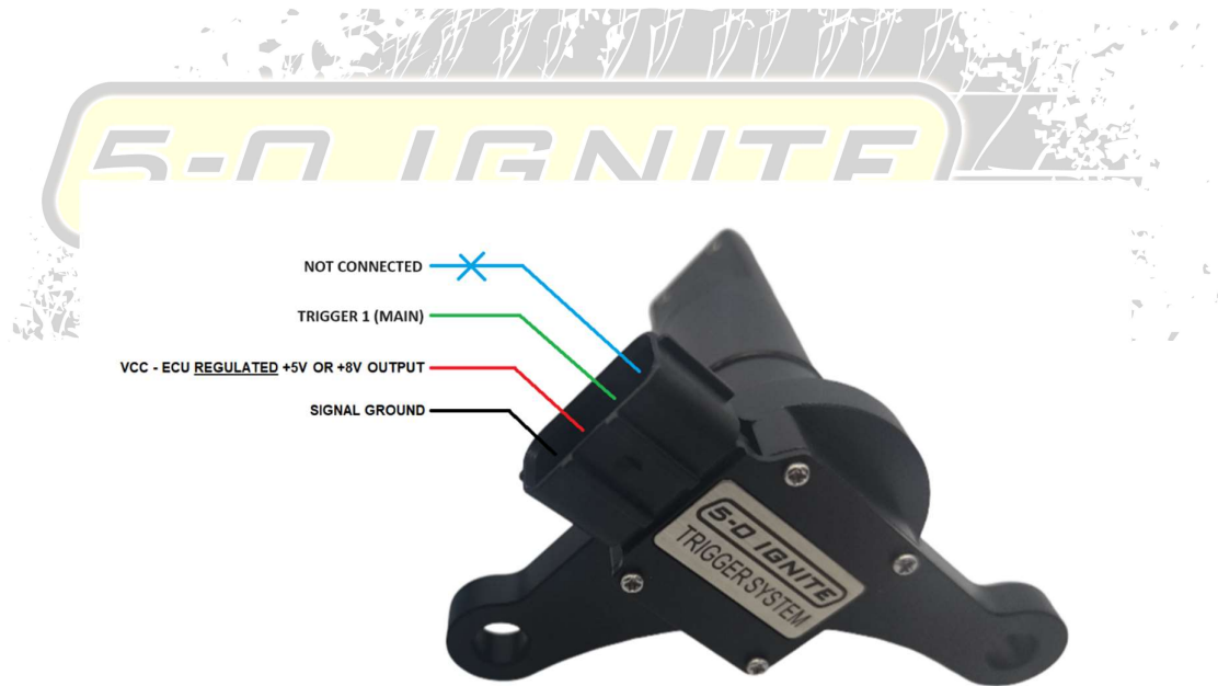
Figure 15 – 5-0 Ignite SR Cam Trigger V3 Sensor Pinout
