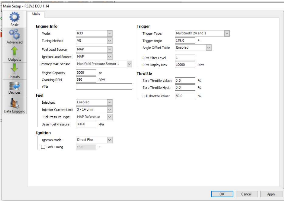
Figure 8 - Haltech Platinum Pro Trigger Configuration Example
