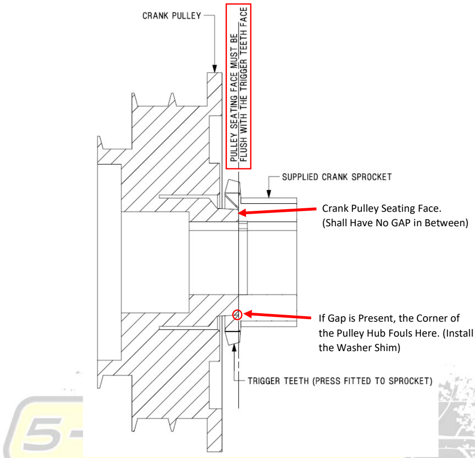
Figure 16 - Pulley Hub Seating Face Shall be Flush with Trigger Teeth Face
