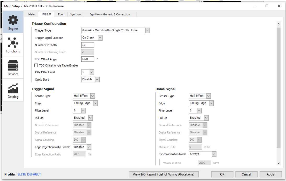
Figure 9 - Haltech Elite Trigger Configuration Example (ESP Software)
