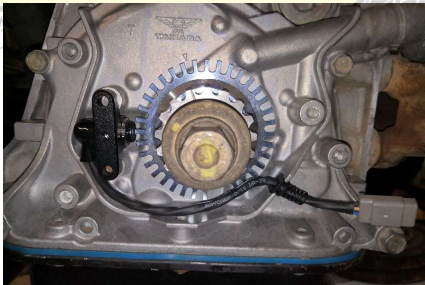
Figure 1 - Install the supplied crank sprocket and crank sensor
