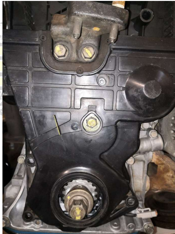
Figure 7 - Install the lower timing belt cover
