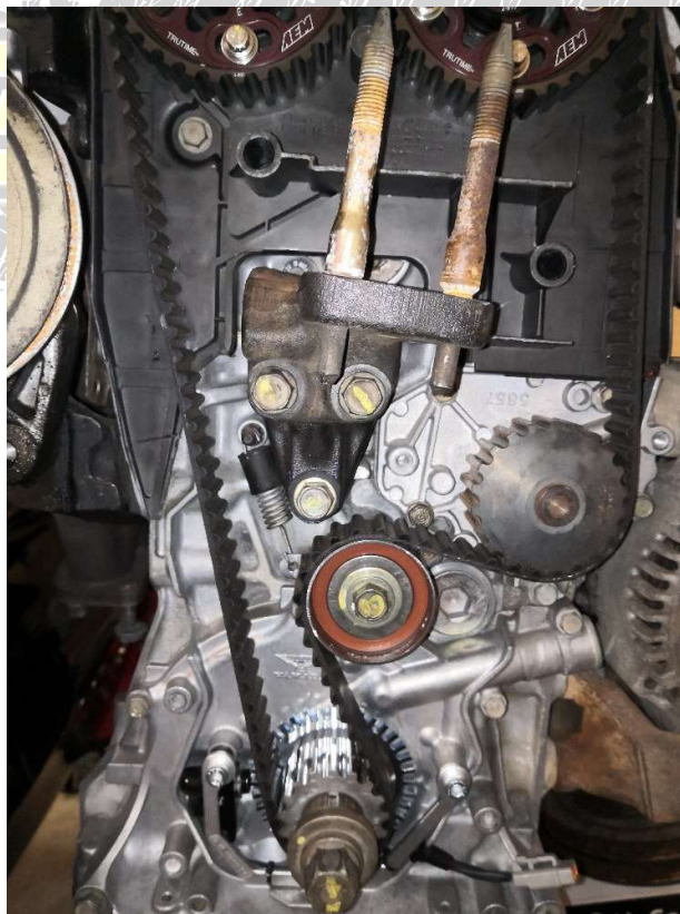
Figure 5 - Install the timing belt
