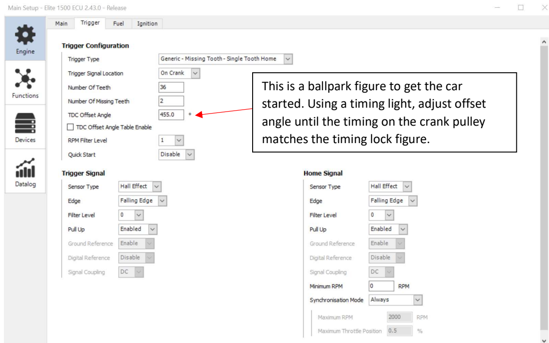
Figure 15 - Haltech Elite ESP/NSP Trigger Settings
