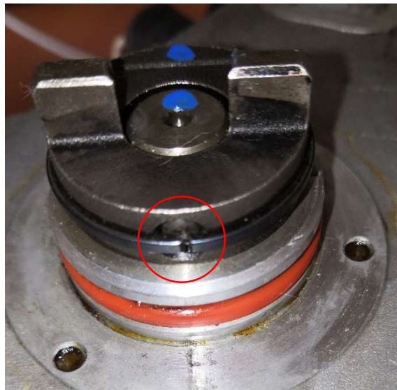
Figure 9 - Rotate c-clip to align with pin hole
