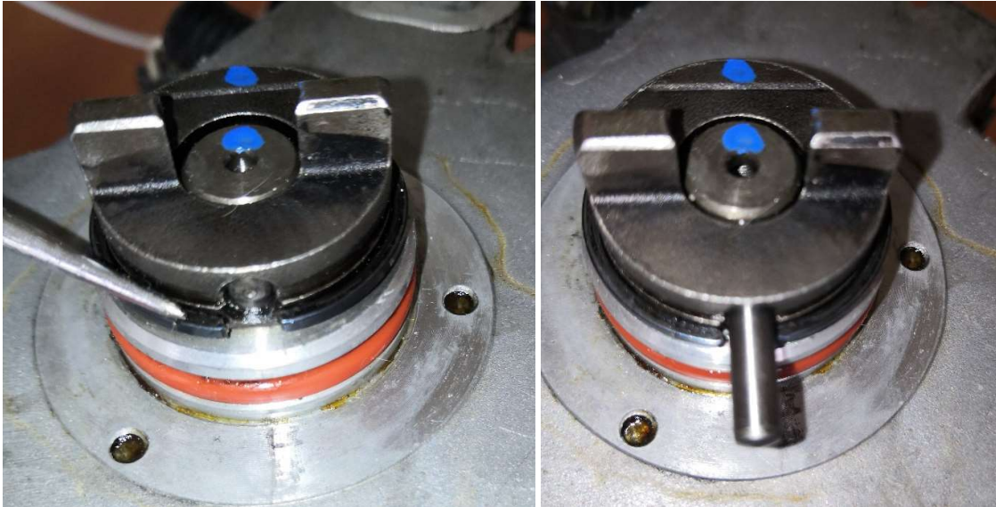
Figure 10 – Slide the pin out and remove the distributor drive key
