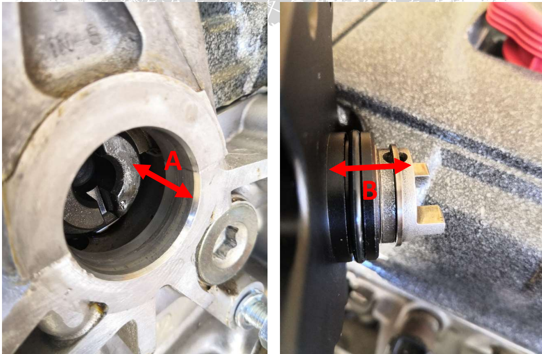
Figure 13 - Camshaft end to key drive clearance check
